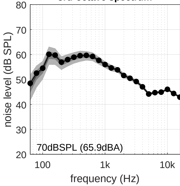
3rd-octave spectrum
